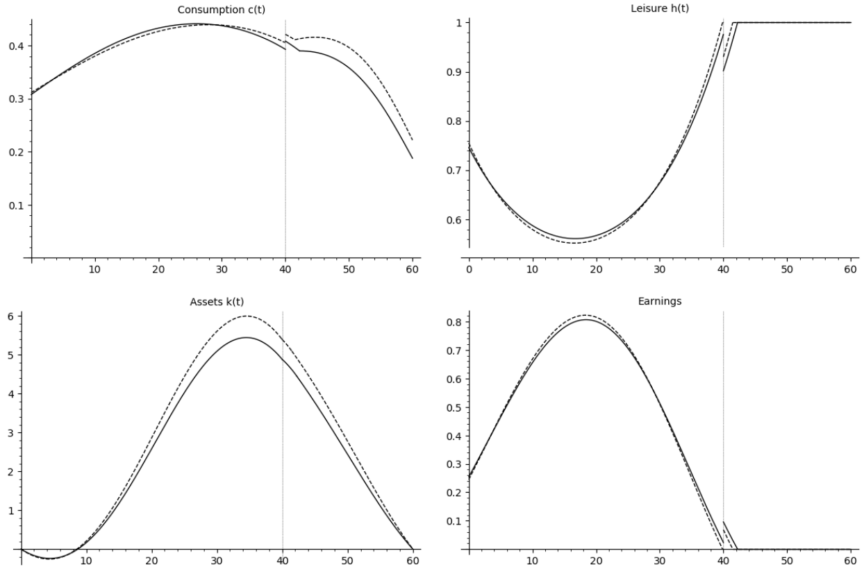
Figure 10: Exponential (solid lines) and hyperbolic (dashed lines) treated profiles ( \beta_1 = 0.2 , \beta_2 = 0.1 ). The value of \tau corresponding to \rho = 0.02 was computed to be 0.0286. r = 3.5\% ; \theta = 0.34 ; \gamma = 2 .
